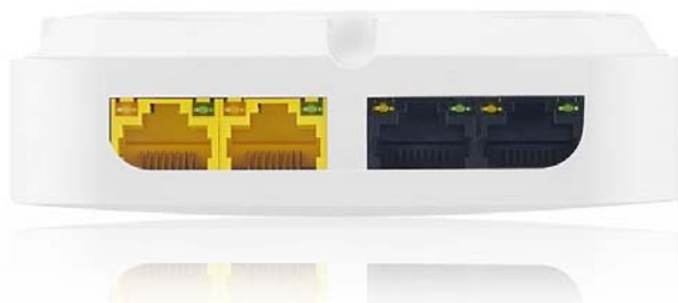
Figure 30 WAX300H Ports
