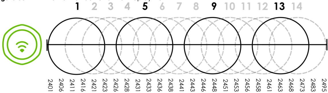
Figure 93 An Alternative Four-Channel Deployment
