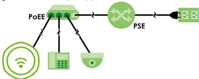
Figure 34 PoE Example Application - PSE with PoE Extender
