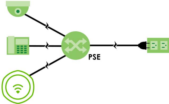
Figure 33 PoE Example Application - PSE
