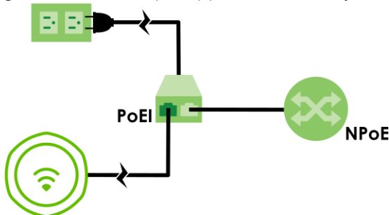
Figure 35 PoE Example Application - PoE Injector
