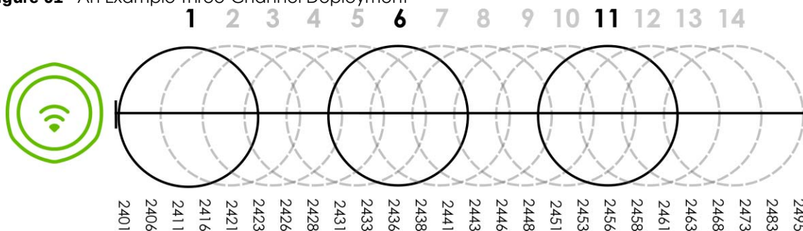
Figure 91 An Example Three-Channel Deployment
